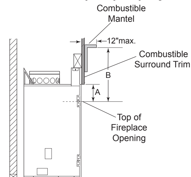
Figure 42 - Locating Mantel
