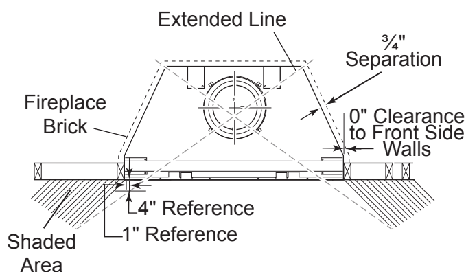
Figure 41 - Front and Side Clearances
