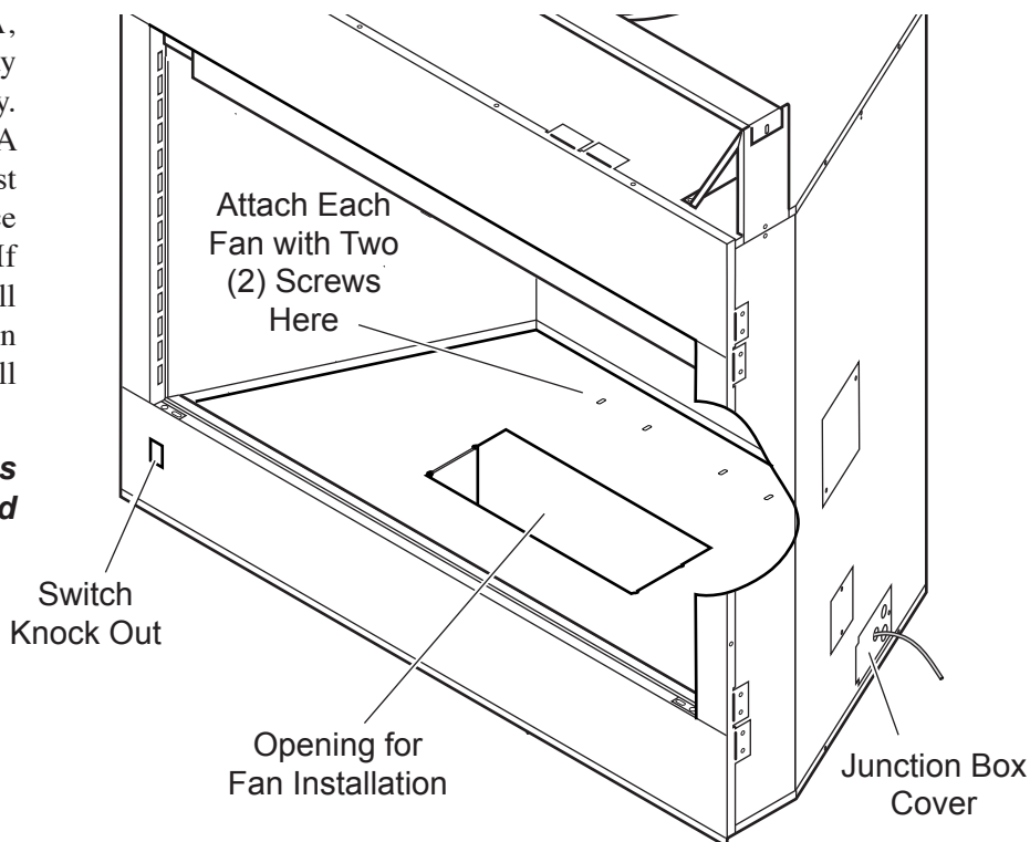
Figure 43 - Blower Location
