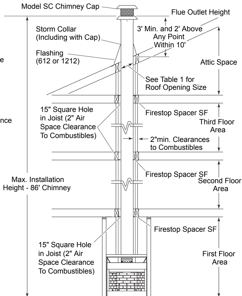
Figure 15 - Residential Installation
