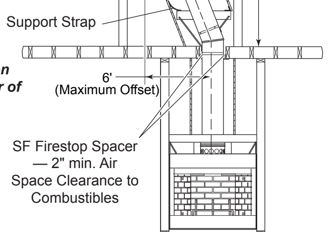
Figure 23 - Installing Chimney with Total Height of Fireplace and Chimney 20' or More
