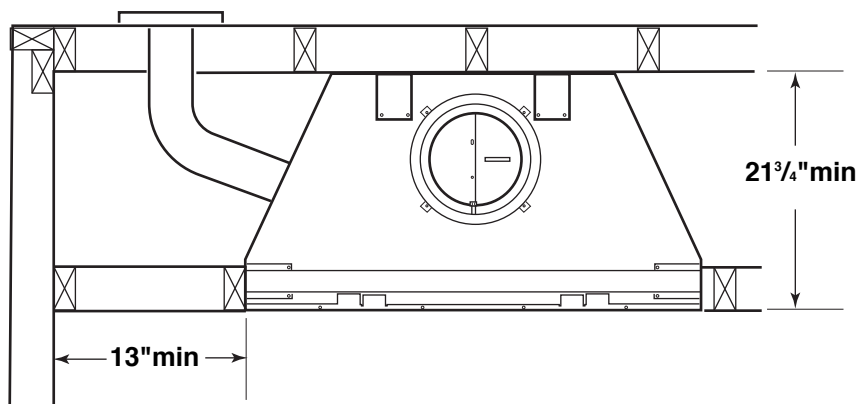
Figure 11 - Minimum Clearances for Wall Installation
