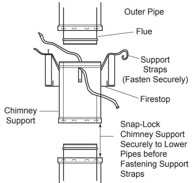
Figure 20 - Installing Chimney Supports
