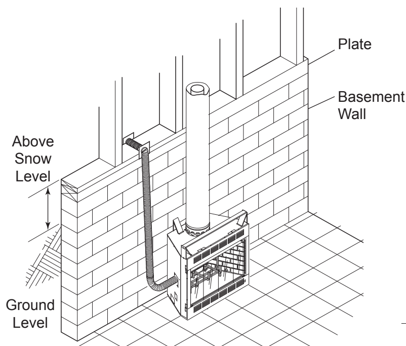
Figure 28 - Basement Installation
