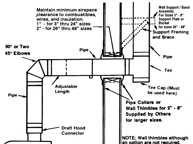
FIG. 7 - WALL PENETRATION FOR TYPE B
