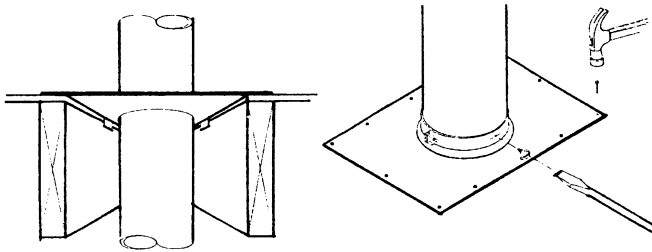
FIG. 9 FIRESTOP/SUPPORT ASSEMBLY
