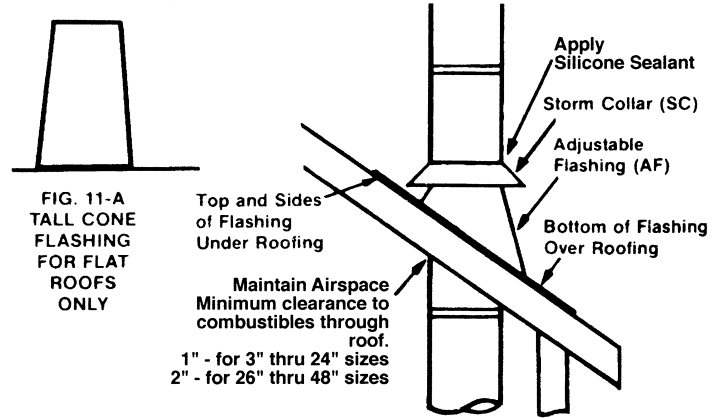
FIG. 11-B ELEMENTS FOR PROPER ROOF FLASHING INSTALLATION
