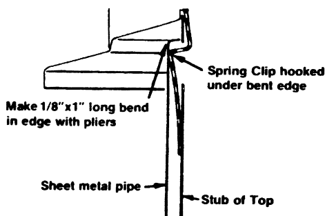
3"-8" TOP INSTALLATION
