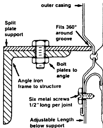
FIG. 10-A SPLIT PLATE SUGGESTED SUPPORT DETAIL
